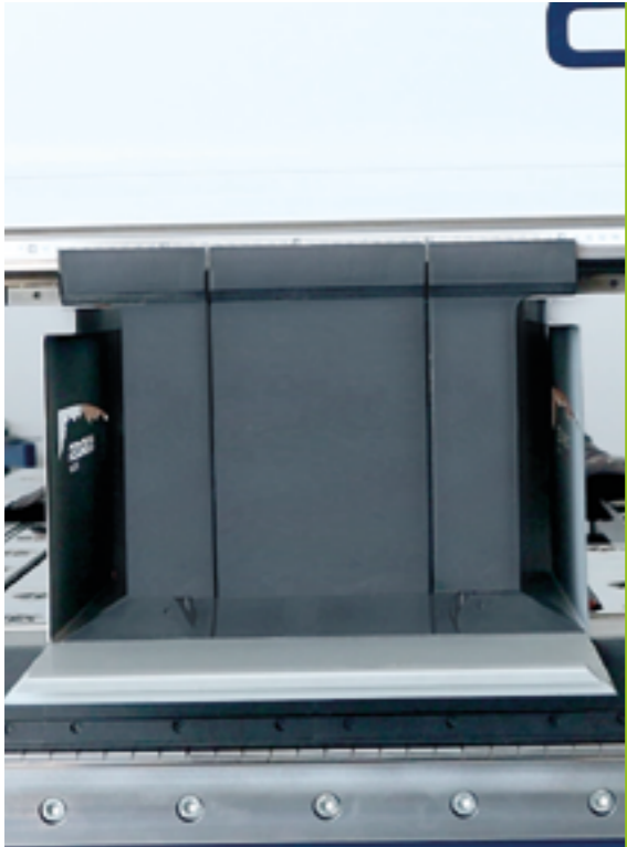
Hydraulic tool clamping and clamping beam stroke of 540 mm for up to 250 mm high products.
