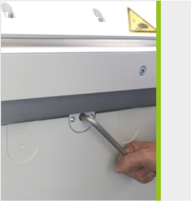
Crowning device for folding beam: manual central crowning device (not in combination with cranked folding blades).
